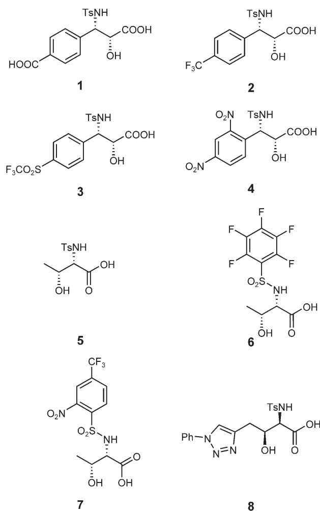
Figure 1. 2 nd cycle ligands used in this study.
