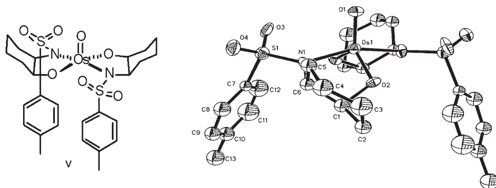
Scheme 2. X-ray crystal structure of osmium bis(azaglycolate) complex V .
