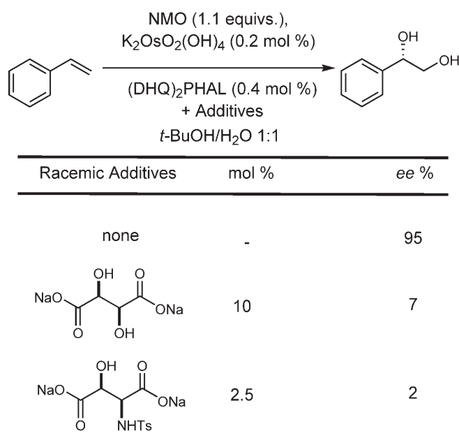
Scheme 3. Effect of racemic additives on enantioselectivity of asymmetric dihydroxylation (AD) of styrene.
