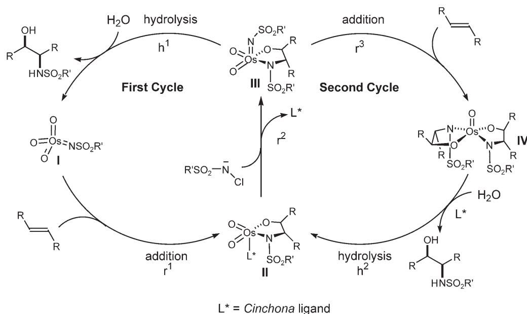
Scheme 1. Two catalytic cycles in aminohydroxylation of olefins.
